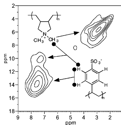
Figure 13. 2D double-quantum back-to-back spectrum of a 3-bilayer film. Auto-peaks and cross-peaks are labeled. The PSS aromatic "auto" peak does not lie on the diagonal because of the different resonance frequencies of the two protons involved.
