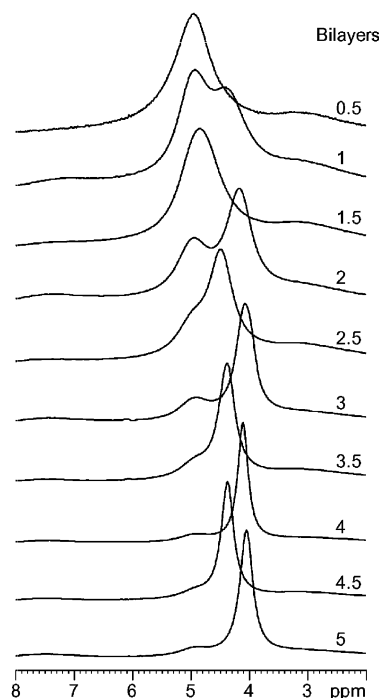
Figure 1. 1 H spin-echo NMR spectra of PEM films equilibrated with atmospheric moisture. The peak at about 5 ppm is water associated with the substrate. The shift of the water associated with the film changes depending on which polymer was last adsorbed. Full bilayers have PSS on the surface. Half bilayers have PDADMAC on the surface.
