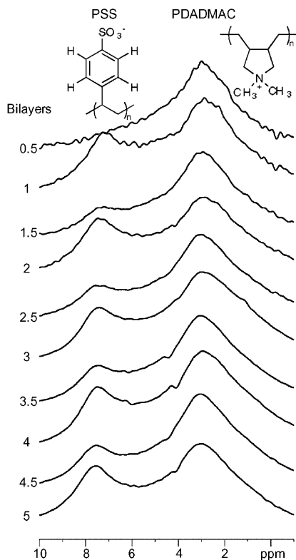
Figure 11. 1D double-quantum-filtered back-to-back spectra (1024 transients) at 40\ \mu\text{s} recoupling time. Note the alternation of the relative intensities of the aromatic PSS peak and the PDADMAC methyl peak. Also note the overall increase in signal-to-noise with an increase in film thickness.
