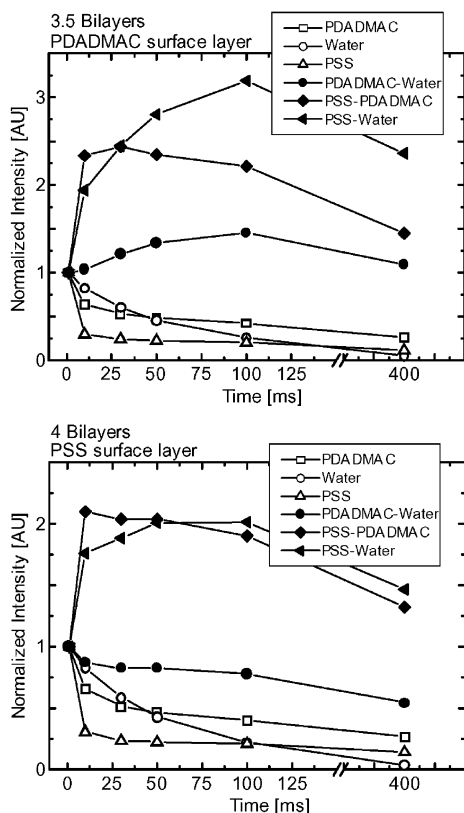
Figure 15. Buildup curves from two series of three-pulse exchange experiments as a function of mixing time (a) for a 3.5-bilayer film with PDADMAC on the surface and (b) for a 4-bilayer film with PSS on the surface. Cross-peaks are solid symbols, and open symbols are diagonal peaks. Integrals at t = 1 ms are set to a value of 1 for ease of viewing. Note that for complete bilayers the water–PDADMAC peak does not build up but rather decays weakly.
