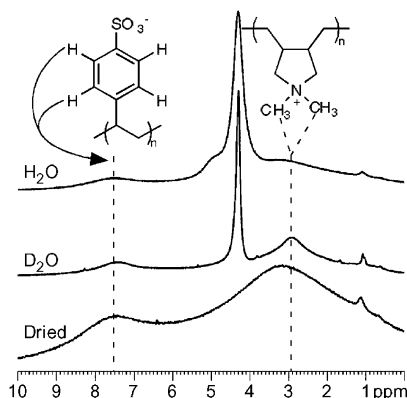
Figure 3. Spin-echo spectra of a 3.5-bilayer PEM film after equilibration with atmospheric moisture ( \text{H}_2\text{O} ), after saturation with \text{D}_2\text{O} , and after drying. Shifts of the aromatic protons of PSS and the methyl protons of PDADMAC are indicated. The residual water peak in the \text{D}_2\text{O} -saturated sample is much narrower than the film water in the atmospheric sample because of a significantly diluted proton dipolar network.
