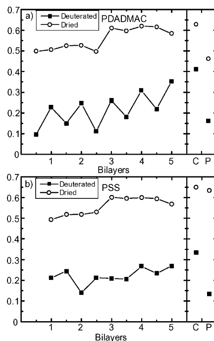
Figure 12. Plot of intensities of (a) the PDADMAC methyl and (b) aromatic PSS regions of the DQF BABA spectra relative to the spin echo for 40\ \mu\text{s} recoupling time. The dried samples (open circles) have been shifted up by 0.25 for clarity. The \text{D}_2\text{O} -saturated samples (solid squares) are samples that have been dried and rehydrated with \text{D}_2\text{O} . C denotes the values for the PEC, and P represents the values for (a) bulk PDADMAC and (b) bulk PSS.
