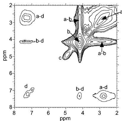
Figure 14. Three-pulse exchange spectrum of a 3.5-bilayer film saturated with D_2O . Observable are the diagonal peaks for (a) the PDADMAC methyl groups, (b) the water associated with the film, (c) the water associated with the substrate, and (d) the aromatic protons for PSS as well as cross-peaks between the polymer components and each polymer with the water associated with the film.
