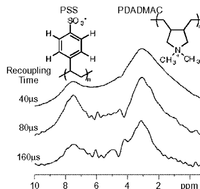
Figure 10. Double-quantum-filtered back-to-back spectra of an atmosphere-equilibrated 3.5-bilayer film. Clearly visible are the aromatic PSS protons and the PDADMAC methyl protons.
