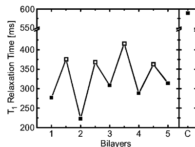
Figure 9. T_1 relaxation times of water in PEMs rehydrated by exposure to atmospheric moisture. C is the measured value for an identically treated PEC. Higher values indicate more mobility (fast-motion limit). Open symbols are samples that have PDADMAC as an outer layer, and filled symbols have PSS as an outer layer.
