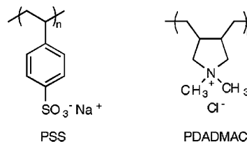
Scheme 1. Polyanion Poly(sodium 4-styrenesulfonate) and Polycation Poly(diallyldimethylammonium chloride)
