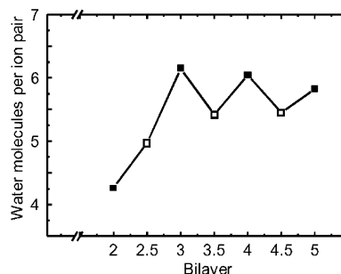
Figure 6. Water content as a function of bilayer number for films equilibrated with atmospheric moisture. Open symbols are samples which have PDADMAC as an outer layer, and filled symbols have PSS as an outer layer. Deconvolution for early layers is hampered by the relative intensity and overlap of the water associated with the substrate; therefore, the plot shows only data for films of 2 bilayers and thicker.
