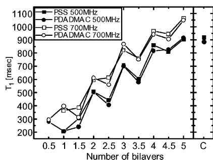
Figure 8. Plot of the spin-lattice relaxation times for D_2O -saturated PEM films. Squares represent the PSS component, and the circles represent the PDADMAC component. Filled symbols were measured at 500 MHz and open symbols at 700 MHz. The C values are for a D_2O -saturated PEC at 500 MHz. Higher values indicate more restricted motion (slow-motion limit).
