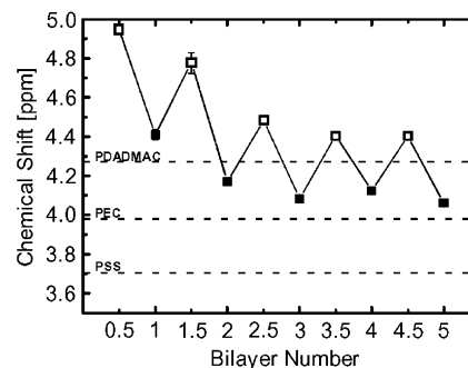
Figure 2. Plot of the chemical shifts of the water adsorbed as a function of bilayer number in PEM films equilibrated with atmospheric moisture. Open symbols are samples which have PDADMAC as an outer layer, and filled symbols have PSS as an outer layer. In addition, the shifts of water associated with the bulk polymers and polyelectrolyte complex are indicated with dashed lines.
