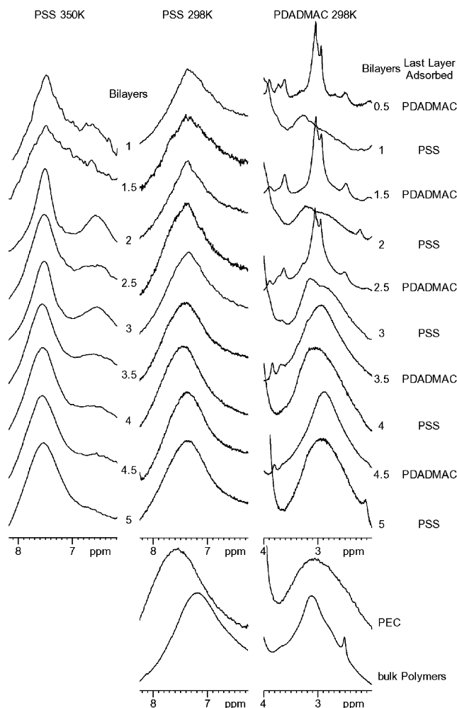
Figure 7. Close-up of the PSS and PDADMAC region at 298 K of the spectra of D_2O -saturated samples. The narrow lines indicate increased motion for the PDADMAC samples when it is the last layer adsorbed. The narrowing of the PSS is not as pronounced. Also shown are the same regions for the PEC and bulk polymers. On the left is the PSS region for the same samples at 350 K.
