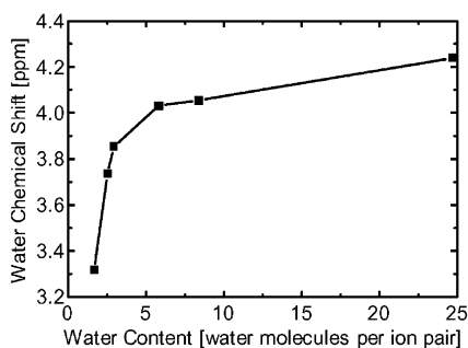
Figure 5. Water chemical shift as a function of water content for a 5-bilayer film.
