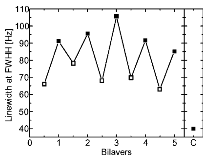
Figure 4. Line width in hertz measured as the full width at half-maximum intensity for samples saturated with \text{D}_2\text{O} . Open symbols are samples that have PDADMAC as an outer layer, and filled symbols have PSS as an outer layer. C indicates the line width of water associated for an identically treated PEC.
